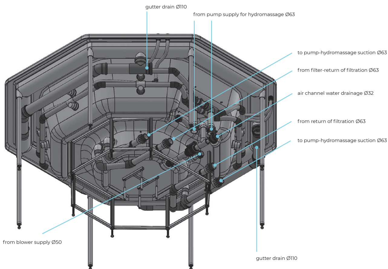
Plumbing scheme for a SPA bathtub with a gutter and a double number of jets, as found in the Vesta bathtub.
