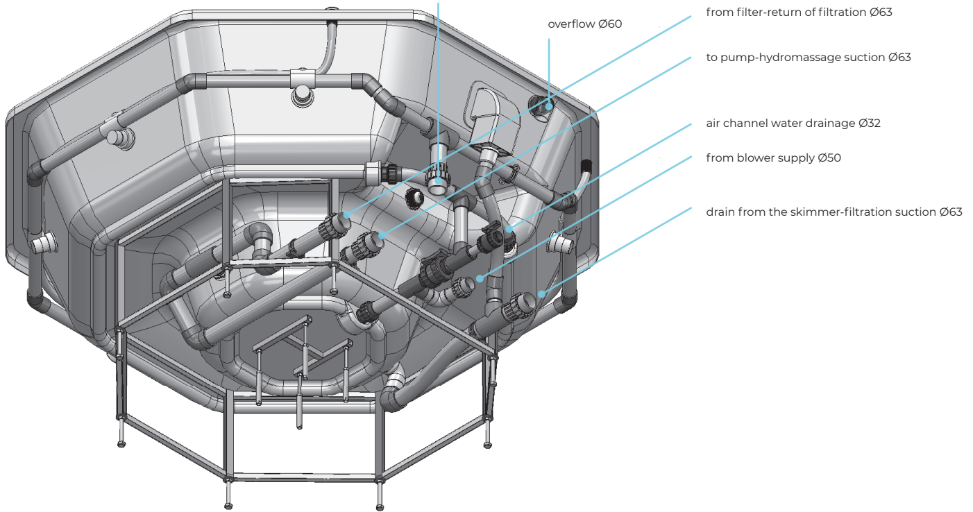
Plumbing scheme for a SPA bathtub with a skimmer and a single number of jets, as found in the Vesta bathtub.
