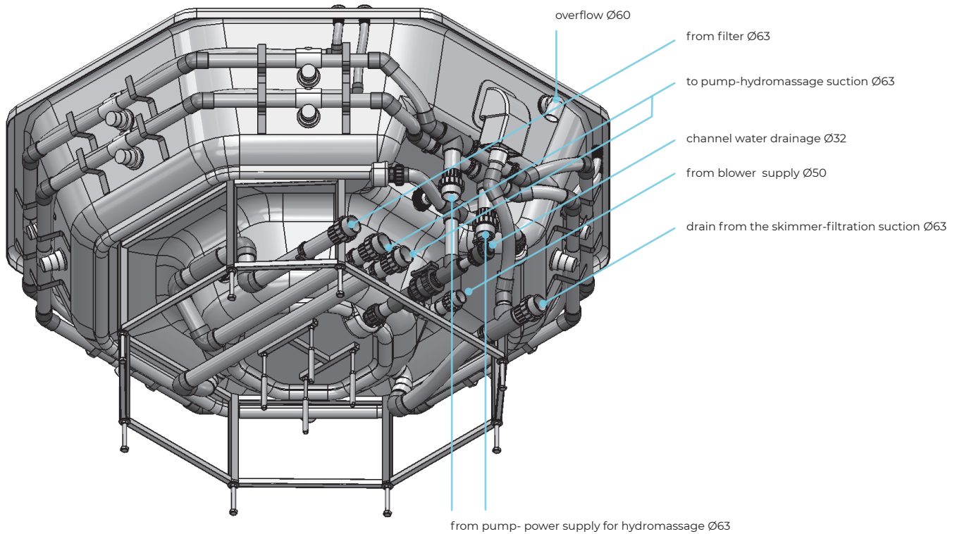
Plumbing scheme for a SPA bathtub with a skimmer and a double number of jets, as found in the Vesta bathtub.
