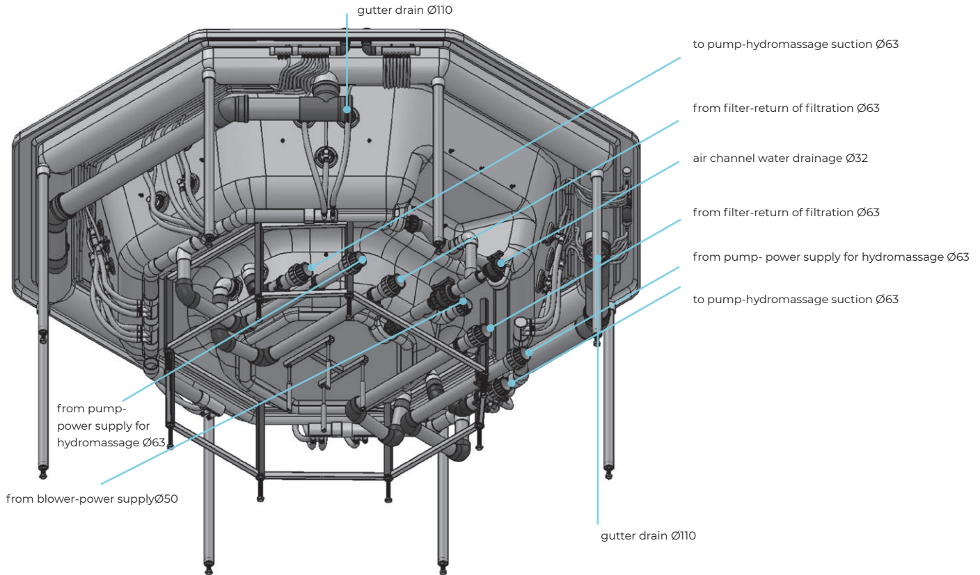
Plumbing scheme for a SPA bathtub with a gutter and 32 jets, as found in the Vesta bathtub.
