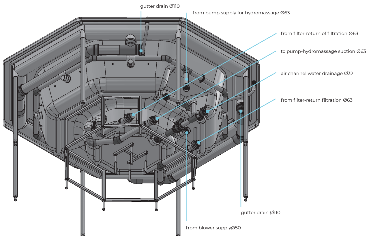
Plumbing scheme for a SPA bathtub with a gutter and a single number of jets, as found in the Vesta bathtub.
